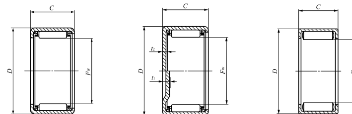
BA...Z BHA...Z
