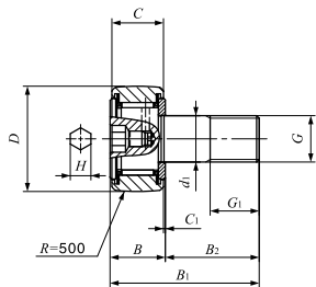
CF...FWBR
