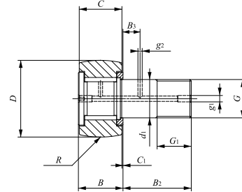
CRH...VR
