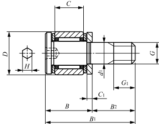
CFS...FW
