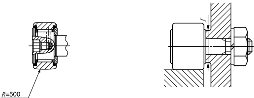
CF...FWBUUR
