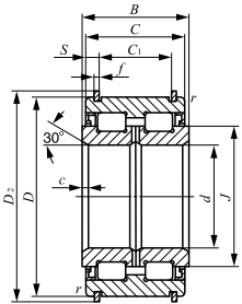
NAS50··ZZNR
