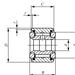
CRY...VUU
